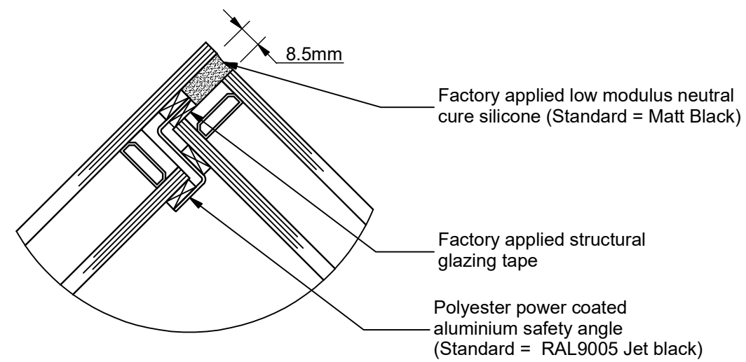
Detail B ( Scale 1 : 2 )
