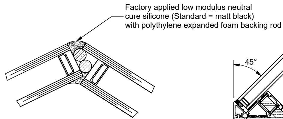
Section C-C through corner join detail (Scale 1:2)
