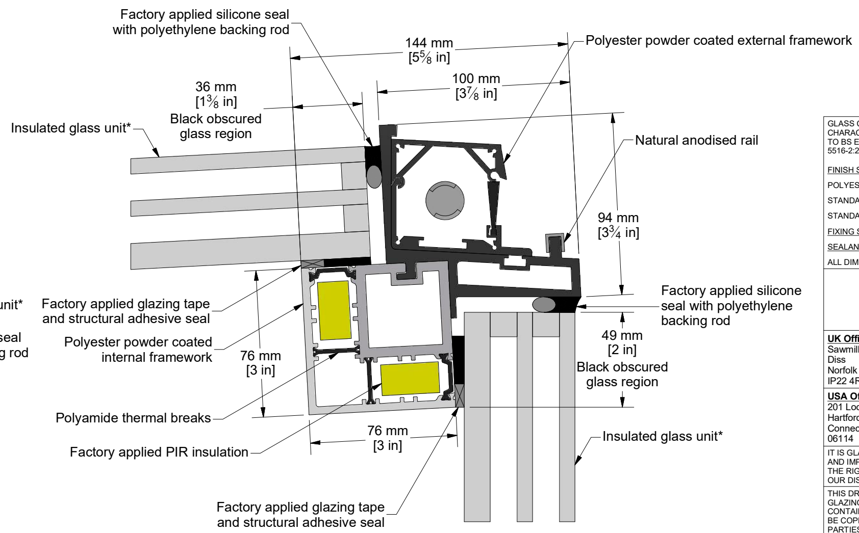
Detail H ( Scale 1 : 2 )
