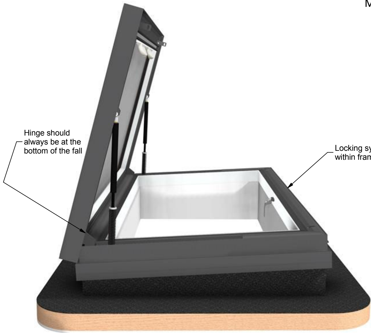
Mechanism detail view Concealed mechanism for assisted opening. Side-mounted pair allow unobstructed views through the leading edge.
