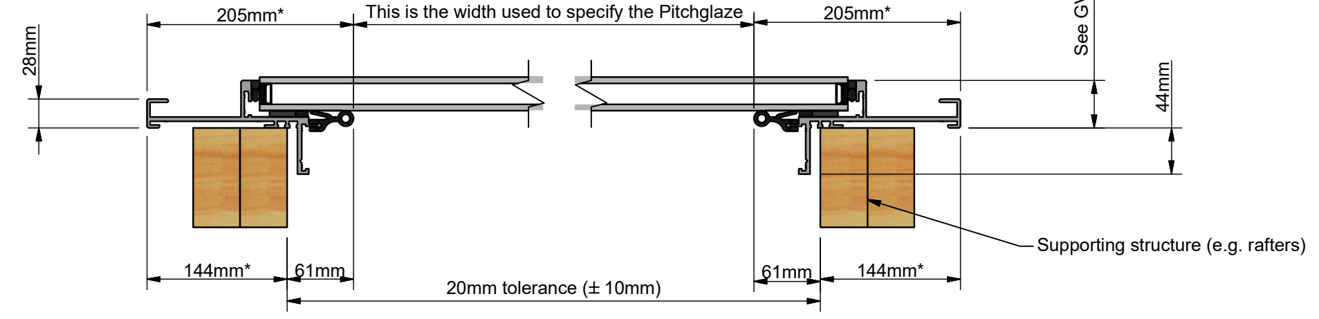
Section B-B OUTSIDE Internal Viewable Width
