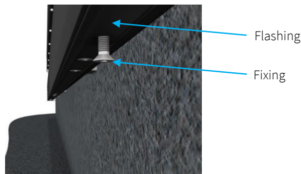
Figure 13 – Flashing fixings
