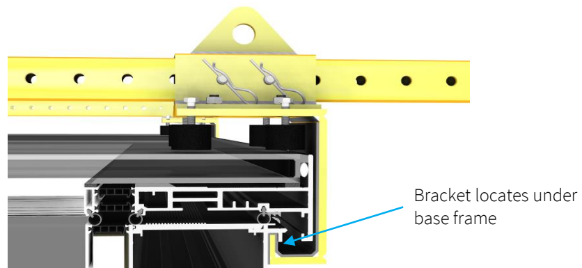
Figure 5 - Locating position
