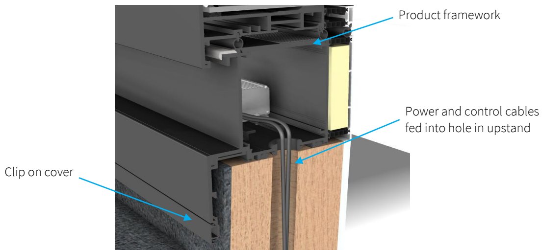
Figure 9 - Position of power and control cables in motor housing
