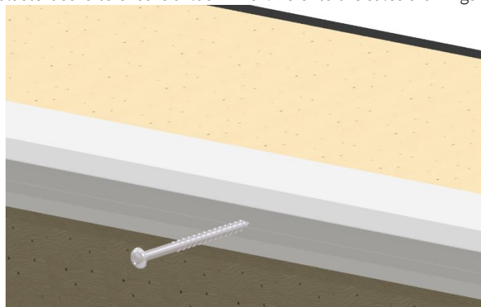
Figure 3 – Upstand top trim fixings
