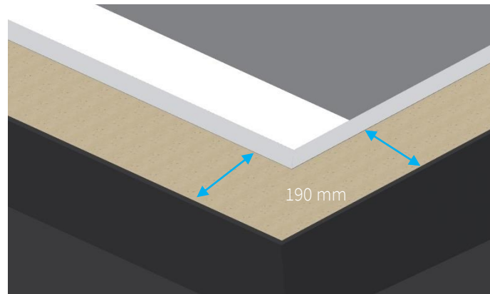
Figure 2 – Upstand top trim measurements
