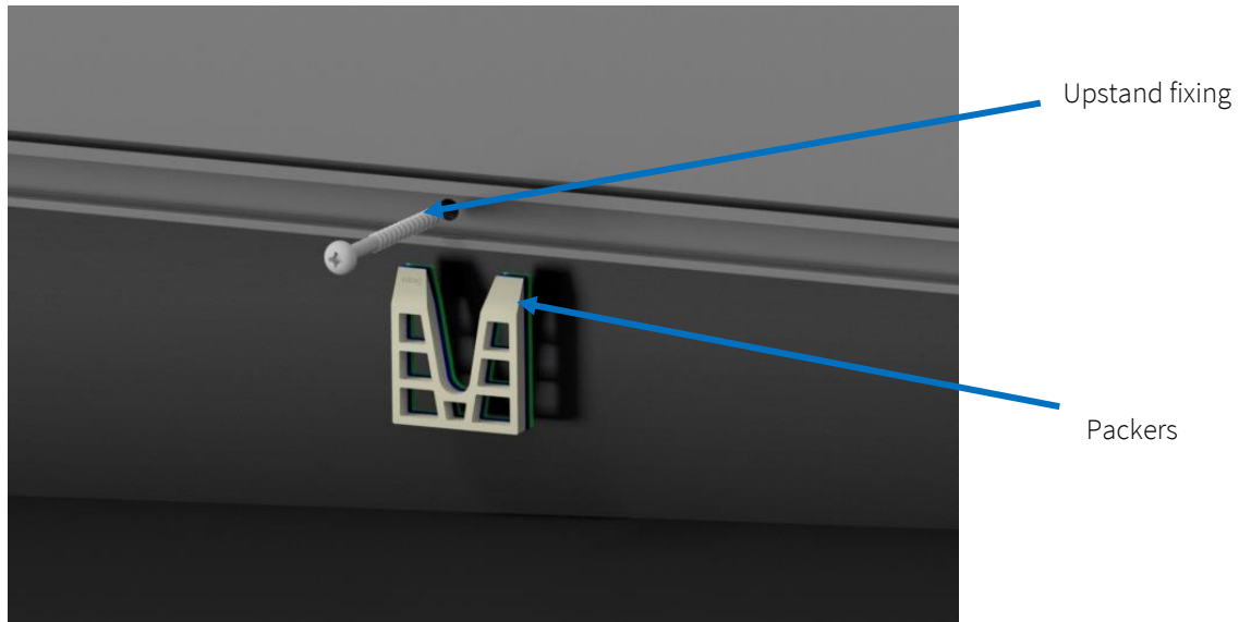
Figure 10 - Upstand fixings
