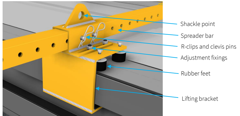
Figure 4 - Lifting bracket
