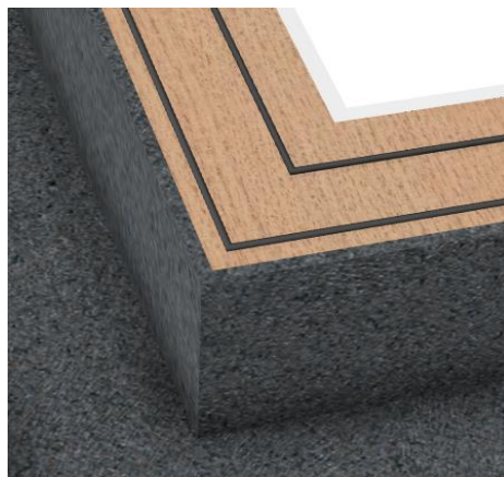
Figure 7 - Silicone/ butyl placement
