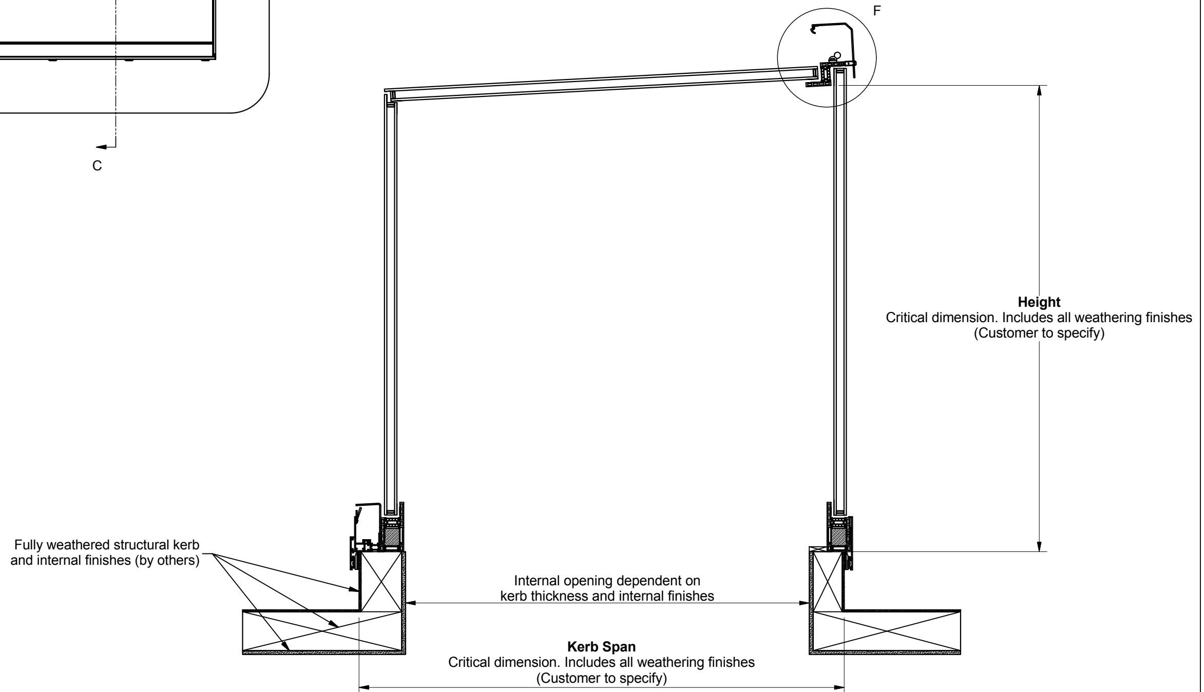
Section C-C ( Scale 1:10 )
