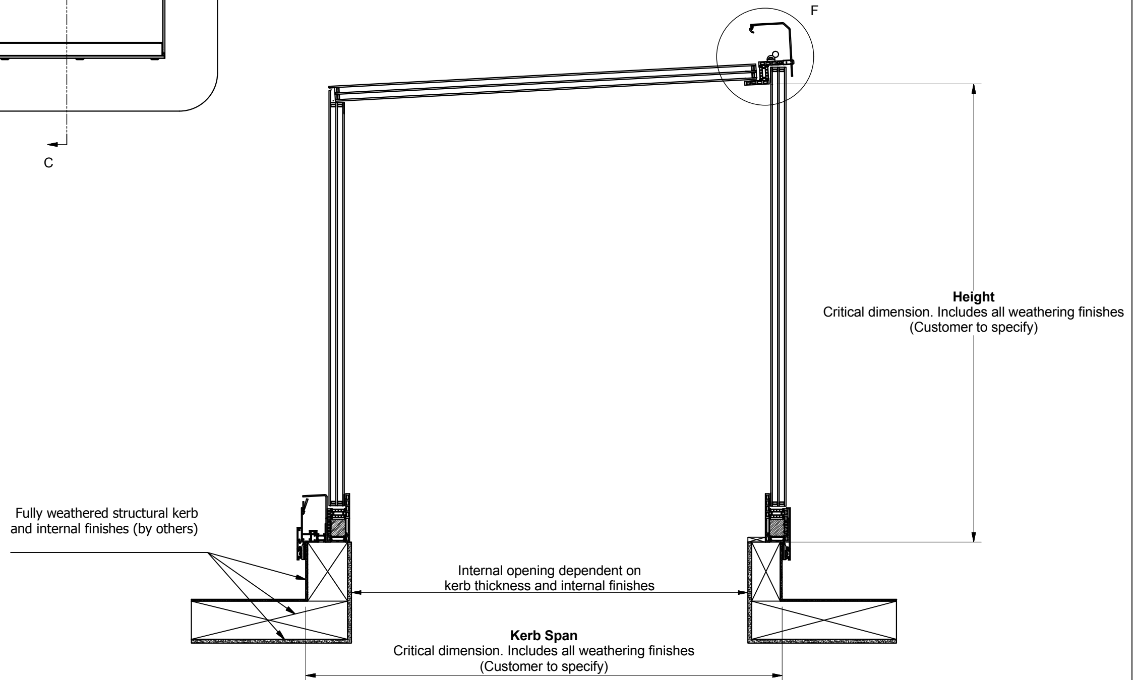
Section C-C ( Scale 1:10 )
