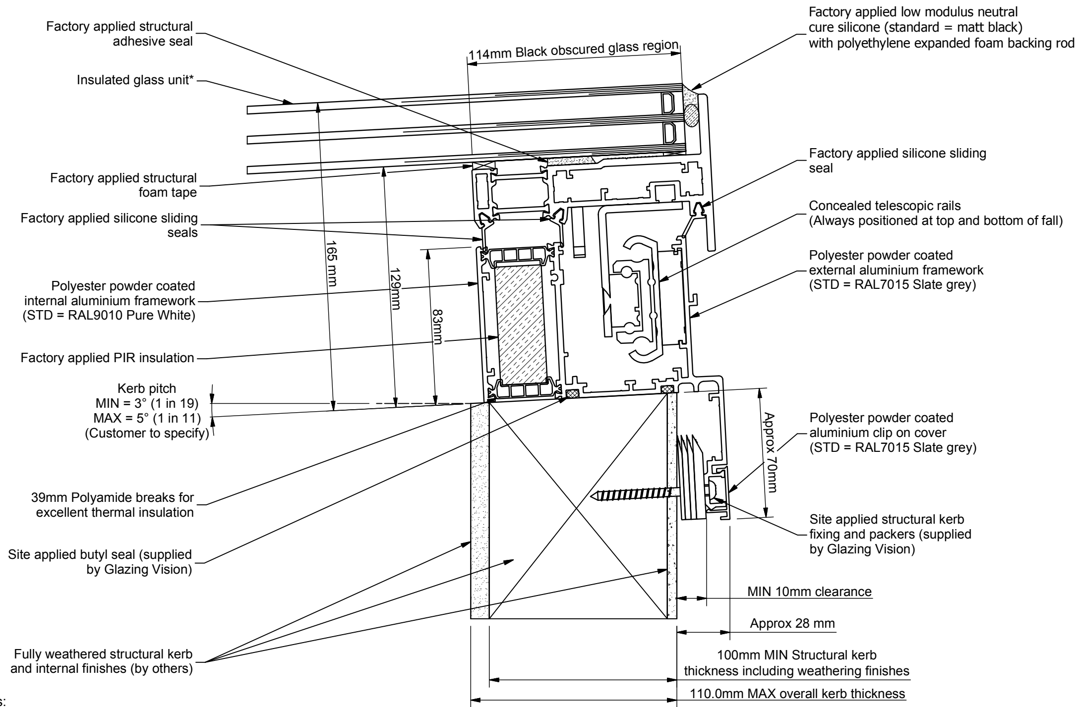
Detail C ( Scale 1:2 ) Section through top of fall
