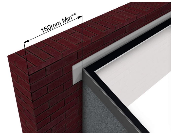
Wall abutment inset detail (NTS)
